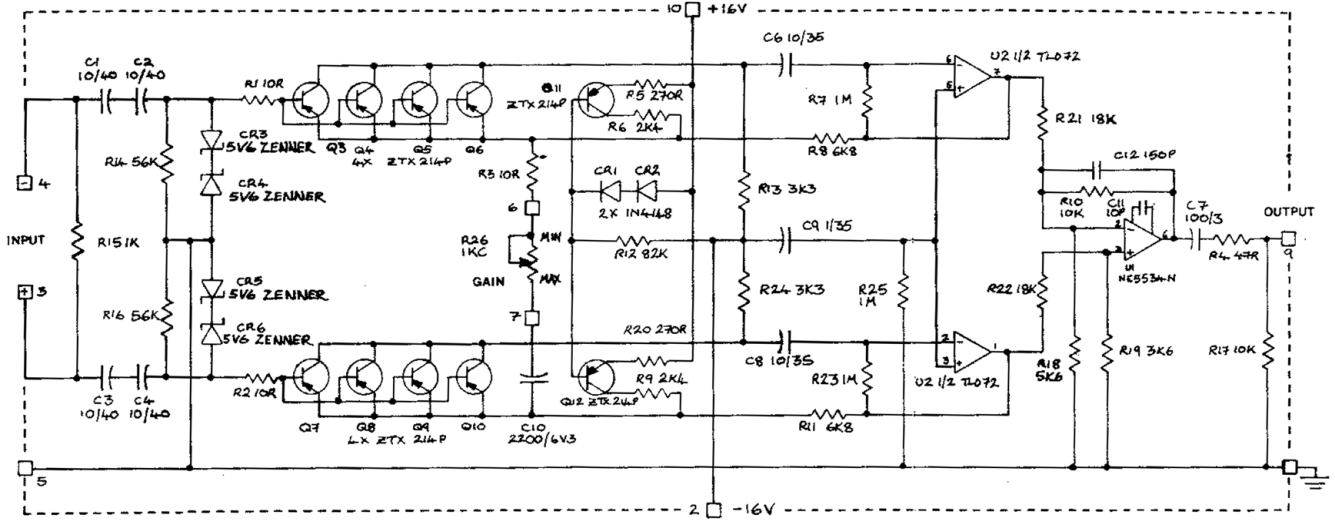
Amek M-2500 microphone input
