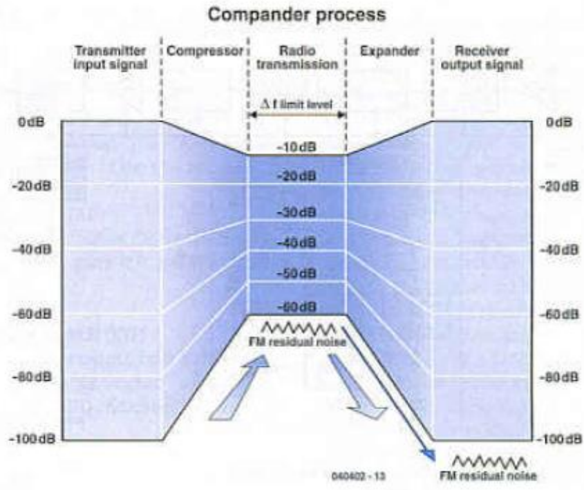
Figure 1. Use of a compander for noise reduction.
